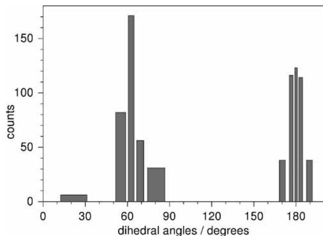
Figure 2. Distribution of K -means clusters of dihedral angles of the conformers of 1,4-BDO. The widths of the bars in the chart are proportional to the standard deviation of each cluster. The - gauche clusters are not shown as they are the mirror images of the + gauche.
